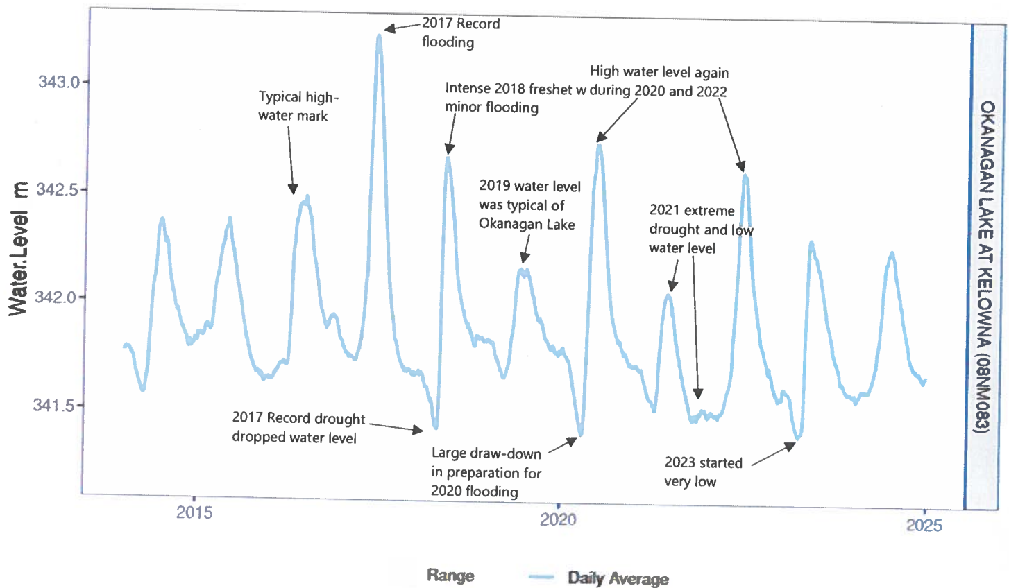
Figure 2: Water level in Okanagan Lake at Kelowna from 2014-2024
