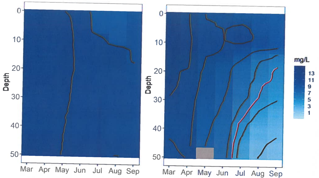
Figure 8: Dissolved oxygen profiles for Okanagan Lake at Summerland (left) and Armstrong Arm (right) during 2024
