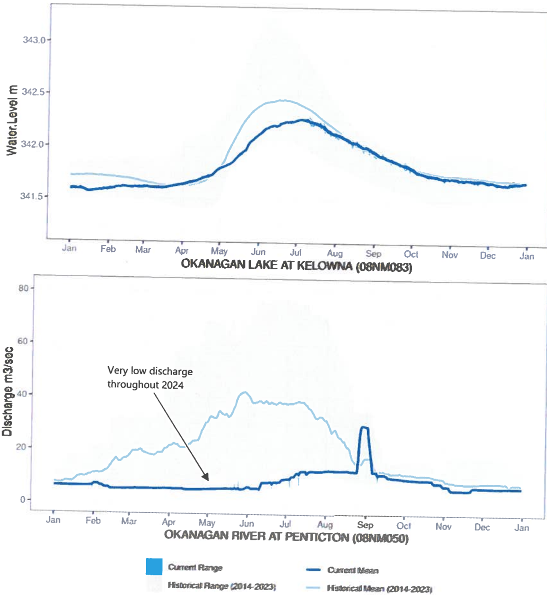
Figure 3: Daily average water level in Okanagan Lake and discharge at Penticton during 2024 compared to previous 10 years Source: (Water Office, 2025)
