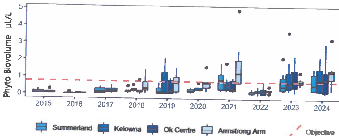
Figure 18: Phytoplankton Biovolume at Summerland and Kelowna, 2015-2024
