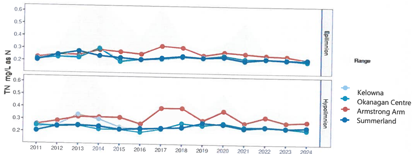
Figure 10: Annual average total nitrogen in Okanagan Lake, 2011-2024
