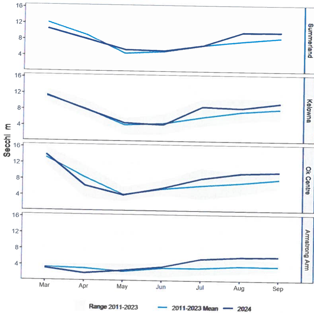
Figure 6: Secchi depth at Okanagan Lake sampling sites during 2024 compared to 2011-2023
