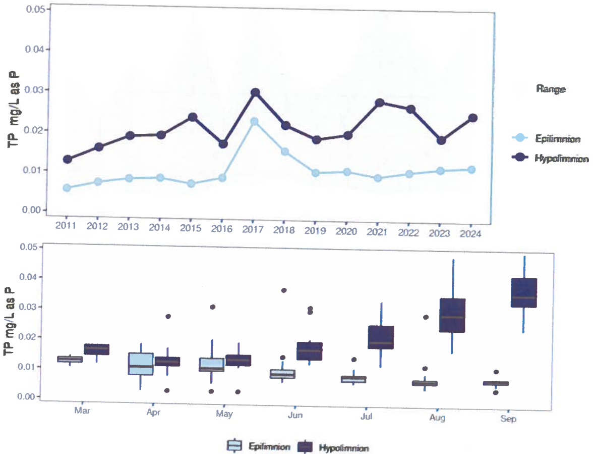
Figure 14: Total phosphorus in the Armstrong Arm, 2011-2024
