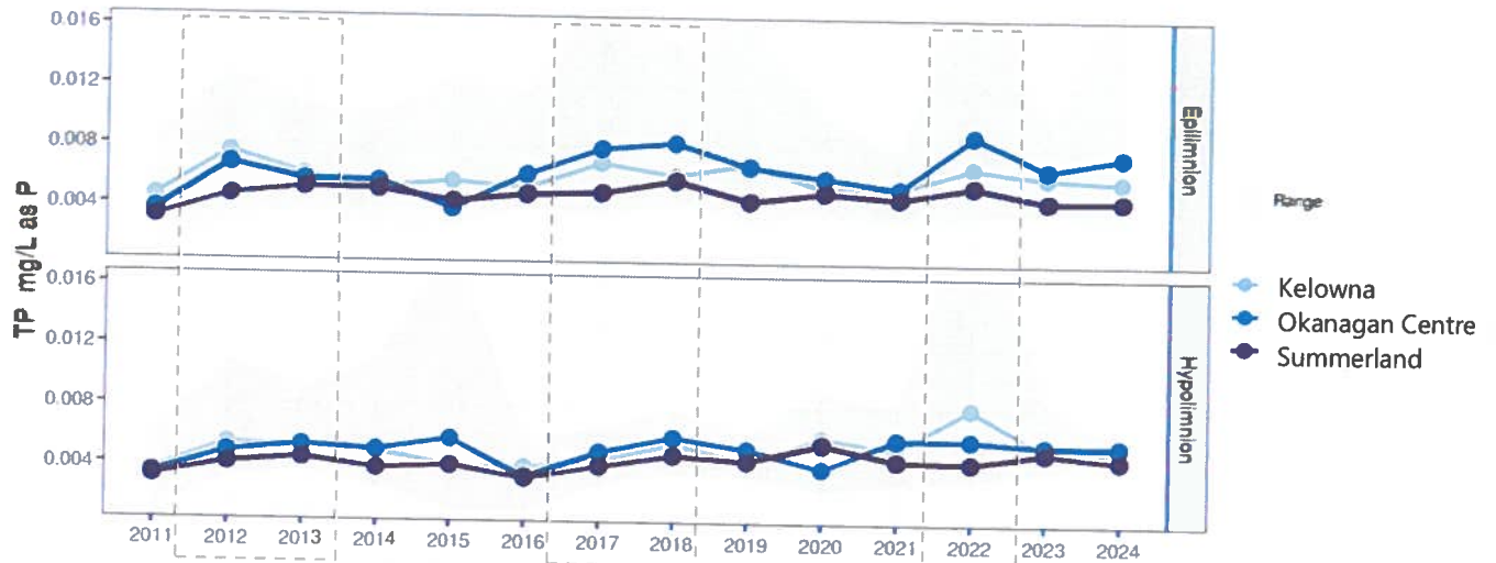
Figure 13: Annual average total phosphorus in Okanagan Lake at the three major basin sampling sites by year from 2011-2024
