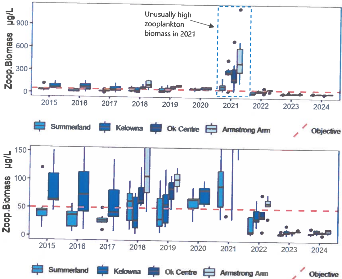
Figure 22: Zooplankton Biomass at the Okanagan Lake sampling locations by year, 2015-2024
