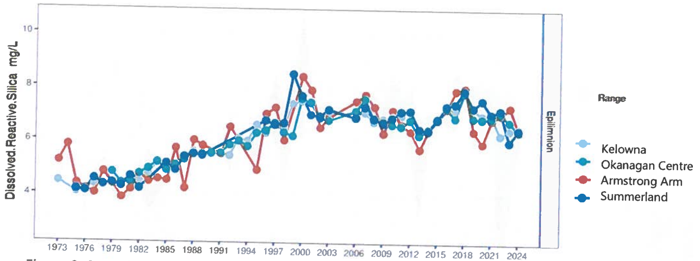
Figure 9: Annual average silica concentration in Okanagan Lake at each sampling site by year with trends highlighted, 1973-2024
