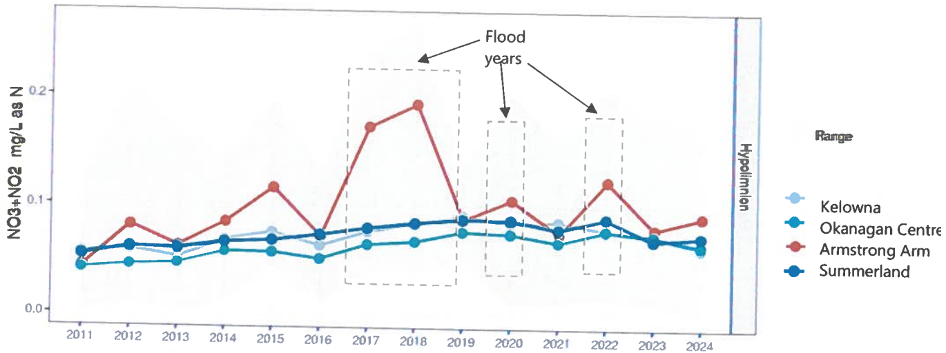
Figure 11: Annual average nitrite (NO 2 ) + nitrate (NO 3 ) in mg/L as N in the deep water of Okanagan Lake, 2011-2024
