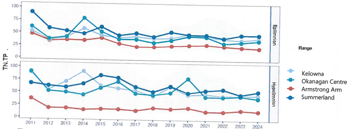
Figure 16: Nitrogen to phosphorus ratio at Okanagan Lake sampling sites 2011-2024
