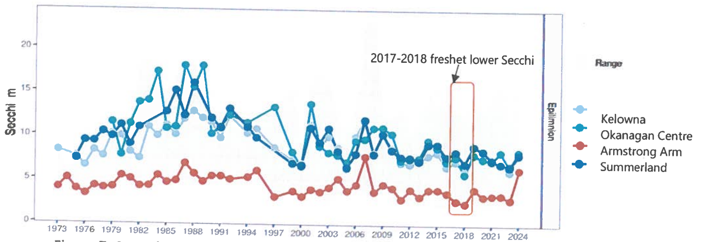
Figure 7: Annual average secchi depth in Okanagan Lake from 1973-2024
