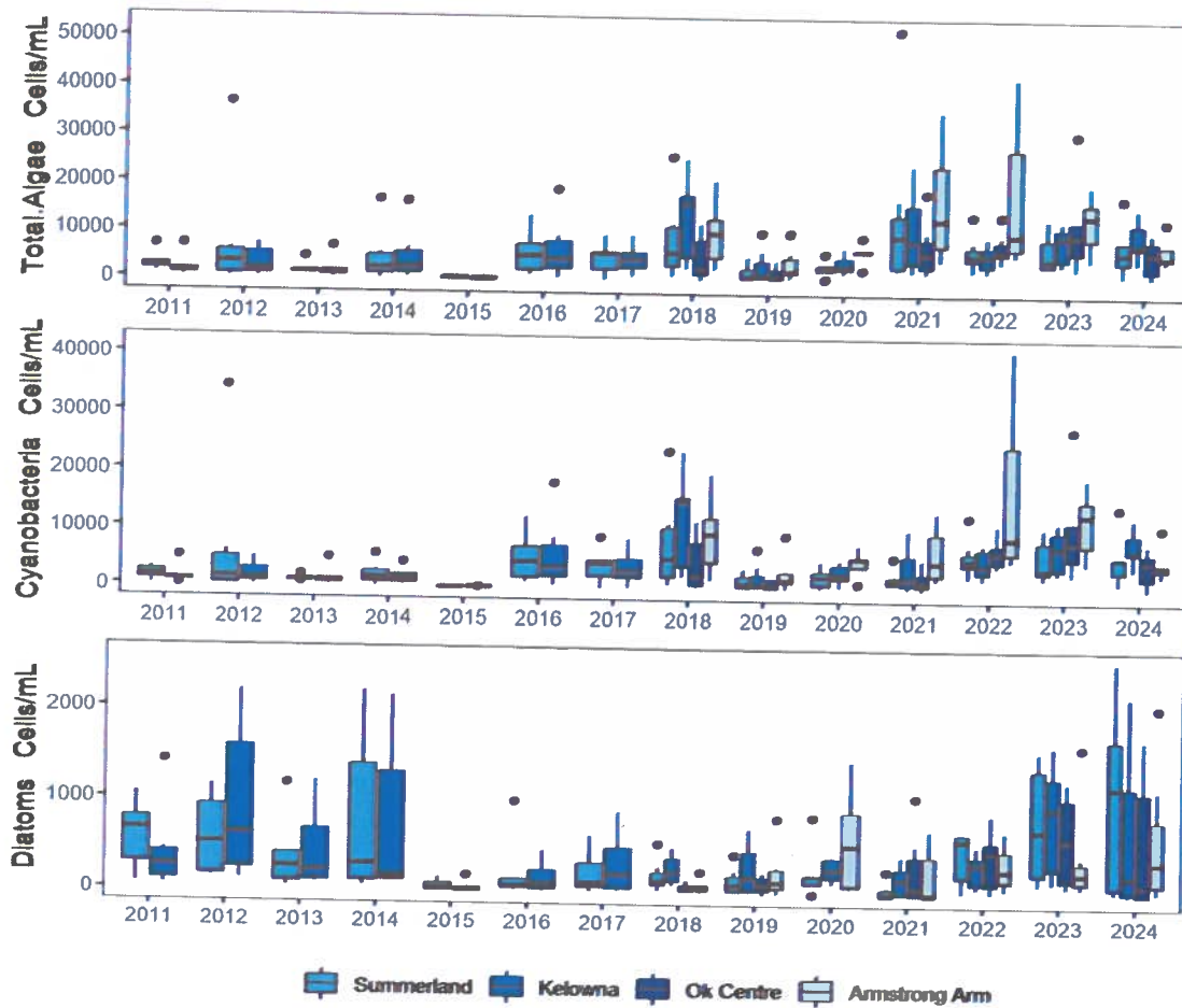
Figure 20: Total algae, cyanobacteria, and diatom counts in Okanagan Lake, 2011-2024
