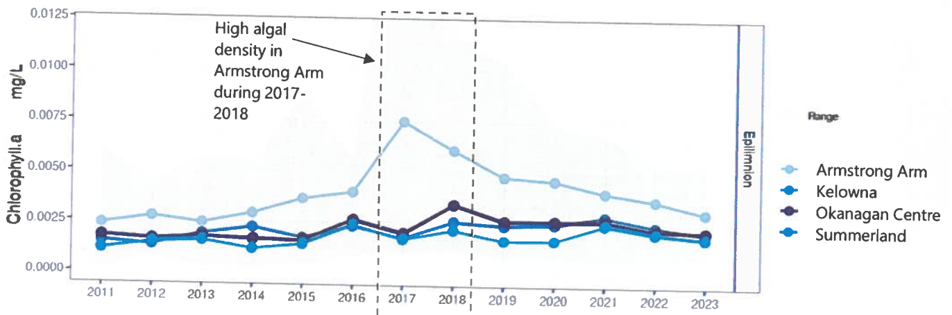
Figure 17: Annual average chlorophyll-a concentration at the four Okanagan Lake sampling sites, 2011-2024
