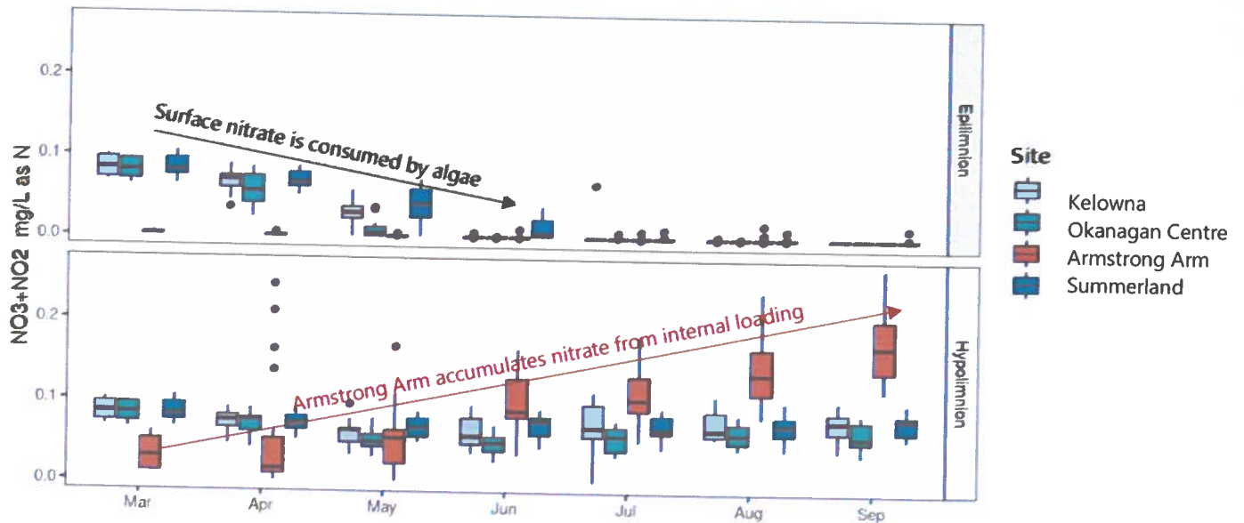
Figure 12: Nitrate + nitrite in Okanagan Lake month illustrating seasonal patterns, 2011-2024
