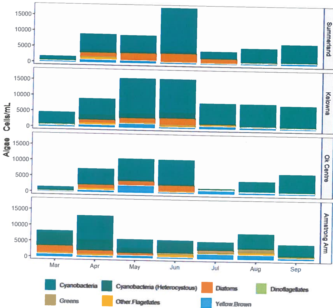
Figure 19: Taxonomic breakdown of algae by major types during 2024
